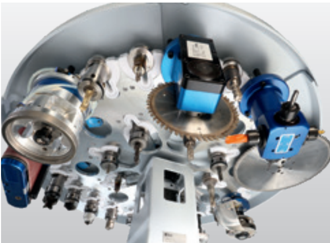
32-space tool changer – arrangement of the tools in an inner and an outer ring. For tools and units with a diameter of up to 200 mm and saw blade up to 350 mm in diameter (in the outer ring).
