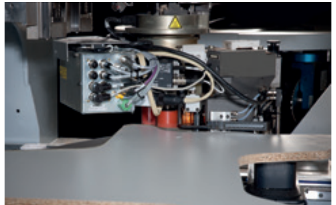
360° edge gluing with the powerEdge edge banding unit
