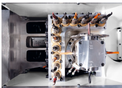
Drilling head V12/H4: HIGH-SPEED drilling head up to 7500 rpm with 12 vertical spindles, grooving saw and 4 horizontal spindles with 0/90° swivel facility. Fast drilling including grooving in the X/Y direction.
