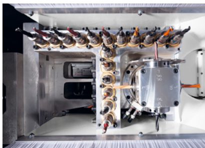
Drilling head V17/H4: HIGH-SPEED drilling head up to 7500 rpm with 17 vertical spindles, grooving saw and 4 horizontal spindles with 0/90° swivel facility. Fast drilling including grooving in the X/Y direction.
