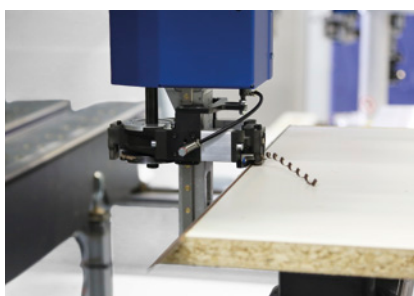
Scraping of mitered edges
