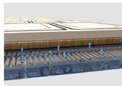
Vacuum grid table with air cushion function: The vacuum transmission is integrated in the design of the aluminium grid table. Division into zones and efficient vacuum pumps ensure reliable clamping, even for nesting processes with underlay panels. The air cushion function makes light work of handling large-format panel-shaped workpieces.
