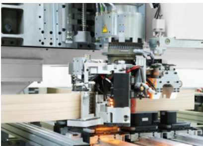
Edge banding for components up to 100 mm in height
