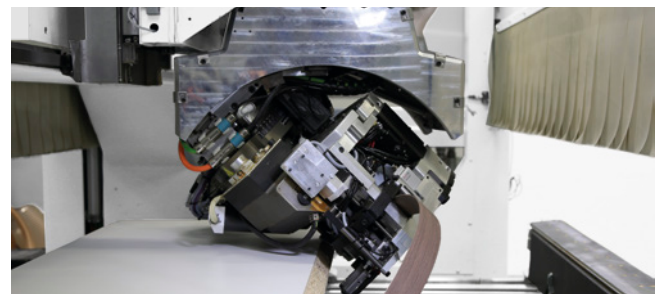
Inclined edge banding: At any optional angle of inclination. The automatic unit adjustment facility allows both shaped edges and inclined edges to be applied to the same workpiece.
