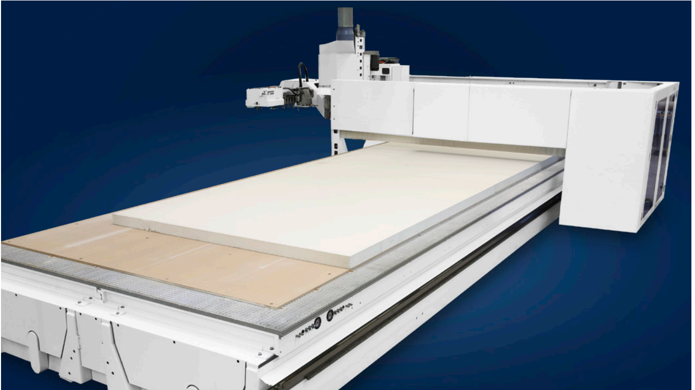
Machine depth XXXL: Components until 3000 mm width for the board processing for construction.
